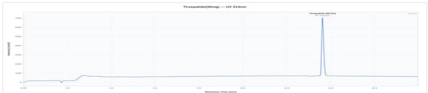
Tirzepatide 30mg - LOT2026-06-0001: UV Chromatogram
