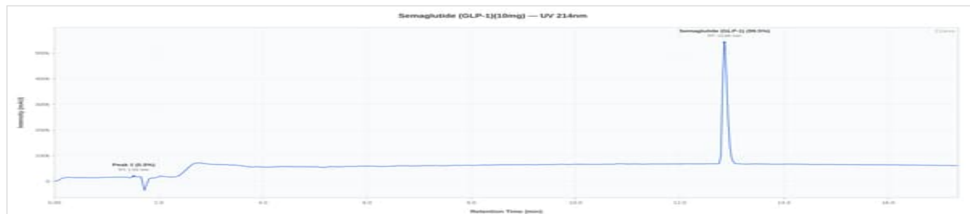
Semaglutide 10mg - LOT2026-06-0001: UV Chromatogram
